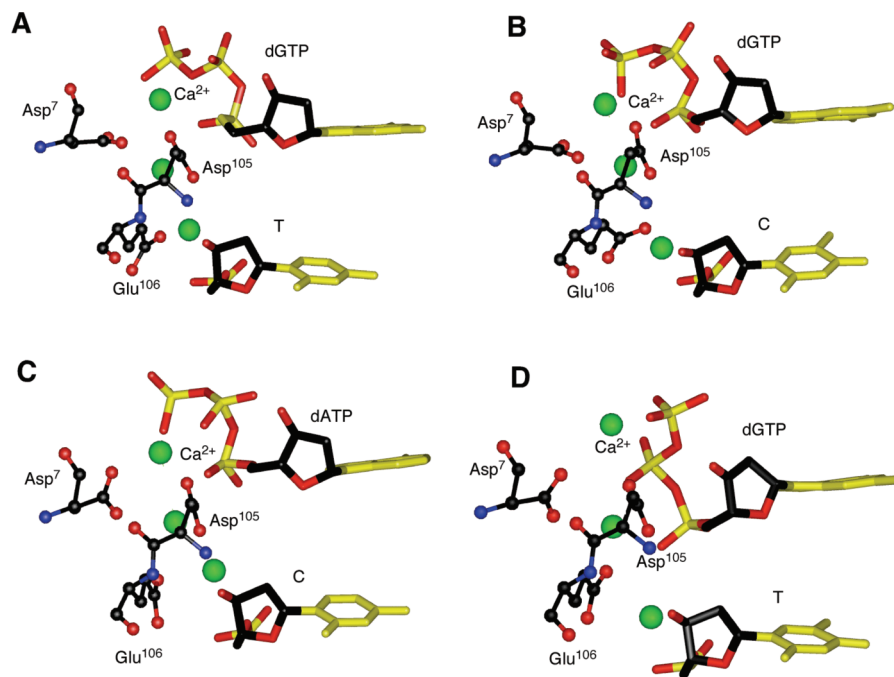
FIGURE 5: Active site structures of three ternary Dpo4–DNA–dNTP complexes containing PdG-adducted DNA, showing the catalytic sites defined by Asp 7 , Asp 105 , and Glu 106 : (A) template sequence I, (B) template sequence II, (C) template sequence III, and (D) type II crystal with native DNA from PDB entry 1JXL (43). The three Ca 2+ ions are shown as green spheres.
