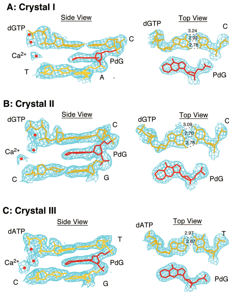
FIGURE 4: Electron density and DNA duplex conformations at the active sites in the three ternary Dpo4–DNA–dNTP complexes: (A) template sequence I, (B) template sequence II, and (C) template sequence III. The views are into the minor groove. Fourier 3F_o - 2F_c sum electron density (light green meshwork) is drawn at the 1\sigma level. Ca 2+ ions and PdG adduct are colored red, and DNA base pairs are colored yellow.
