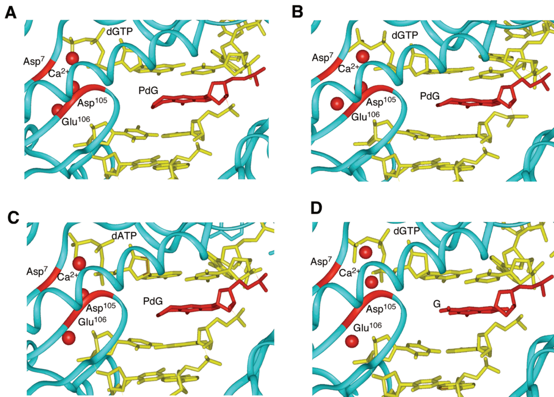
FIGURE 2: Structures of three ternary Dpo4–DNA–dNTP complexes containing PdG-adducted DNA. (A) Template sequence I. (B) Template sequence II. (C) Template sequence III. (D) Type II crystal with native DNA from PDB entry 1JXL (43). The Dpo4 polymerase is colored blue and the PdG adduct red; dNTPs and other DNA bases are colored yellow, and the three Ca 2+ ions are shown as red spheres.
